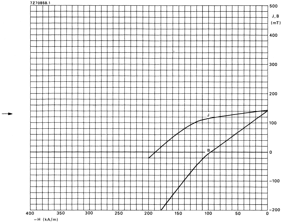
TYPICAL DEMAGNETIZATION CURVE (25 °C)
