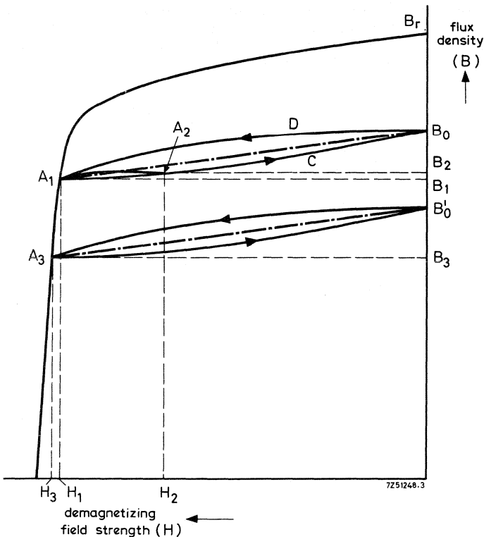
Fig. 4 Recoil lines.
