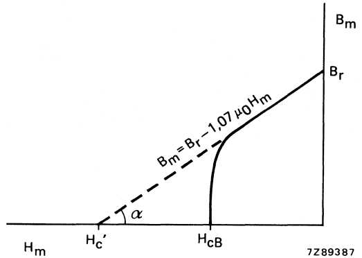
Fig. 3 Demagnetization curve of Ferroxdure.
