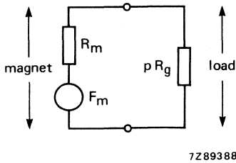
Fig. 2 Equivalent magnetic circuit.
