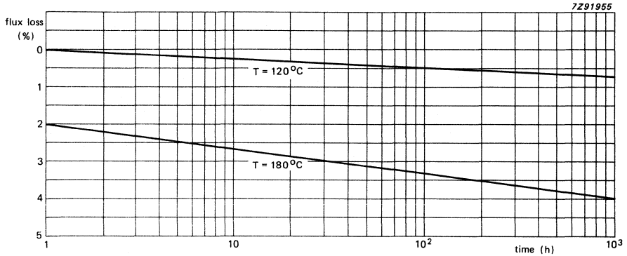
Fig. 9 Irreversible flux losses measured on a disc sample with B/\mu_0H = 1,5 .
