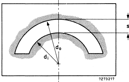
"Go" gauge
